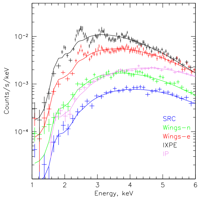
Fig. 4. Background-subtracted Chandra spectra in the vicinity of G0.13–0.11. The colors correspond to the regions shown in Fig. 3 and are identified in this figure. The solid lines show the best-fitting absorbed power-law model fits to these spectra. While a pure power law can describe the compact source spectrum (blue) reasonably well, other regions clearly contain a non-negligible contribution of thermal emission that gives rise to emission lines at low energies. The spectrum of the intermediate polar CXOU GC J174622.7–285218 is shown in purple.
